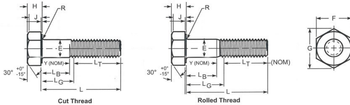
Dimensions of Hex Cap Screws
