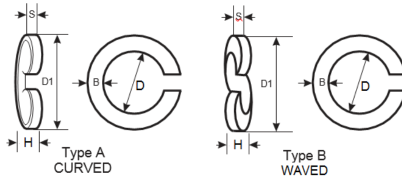
Dimensions of single turn of the spring lock washers DIN 128, Curved Type A
