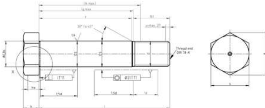
Dimensions of Metric DIN 609 Hex Head Shoulder Screw
