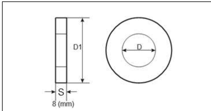
Dimensions of Metric DIN 7989 Thick Flat Washers
