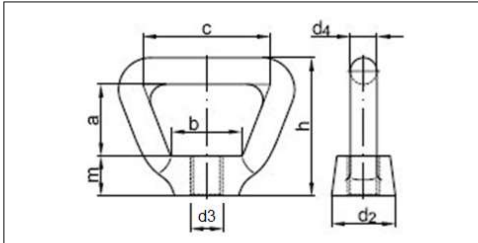
Dimensions and Weight of Metric DIN 80704 Bow Nuts
