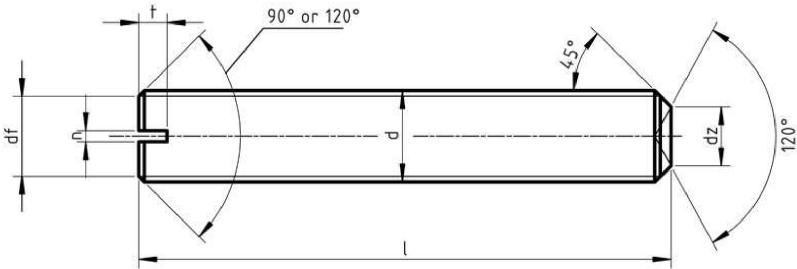
Dimensions of Metric DIN 438 Slotted Set Screws with Cup Point
