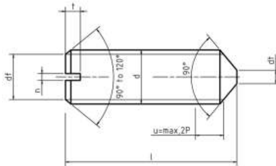
Dimensions of Metric DIN 553 Slotted Set Screws with Cone Point
