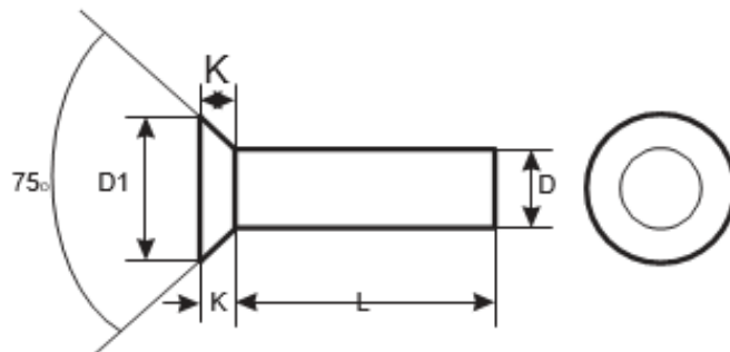
Dimensions of Metric DIN 661 flat countersunk head solid rivets
