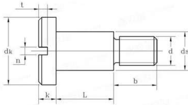
Dimensions of Metric DIN 923 Slotted Pan Head Screws with Shoulder
