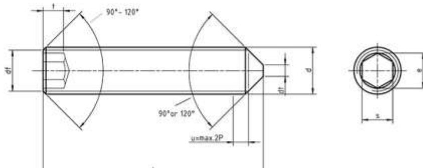
Dimensions of Metric DIN 914 hexagon socket set screws with cone point
